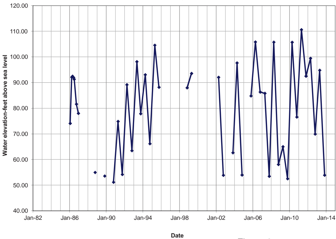
Figure 2 Upper Reach Hydrographs Los Osos Creek
